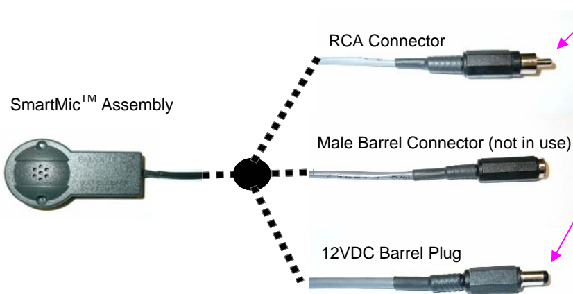
SmartMic Harness (P/N: MICWHAGSRMICCab_XX)
